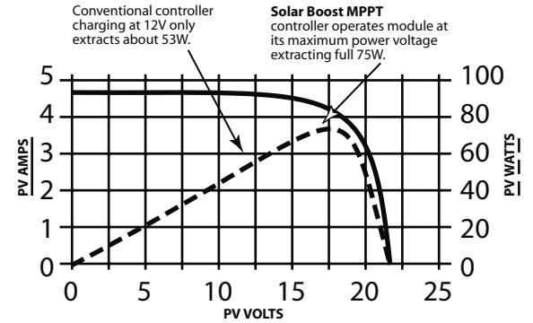
Typical 75W PV Module Performance 25°C Cell • 1000W/m 2
